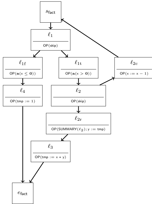
Fig. 6 Control-flow graph of function from Example 4 after the application of TOTALCFL. Note that the choice of \text{SUMMARY}(\ell_2) is not important, as even the summary true suffices to prove termination.
