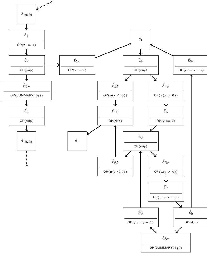
Fig. 5 Control-flow graph from Example 3, which is the output of TOTALCFL when applied to the program in Example 1 and Figure 2. Note that \text{SUMMARY}(\ell_2) and \text{SUMMARY}(\ell_2) both represent commands with the relational meaning equaling x' = x' \wedge y' = y \wedge z' = 0 .
