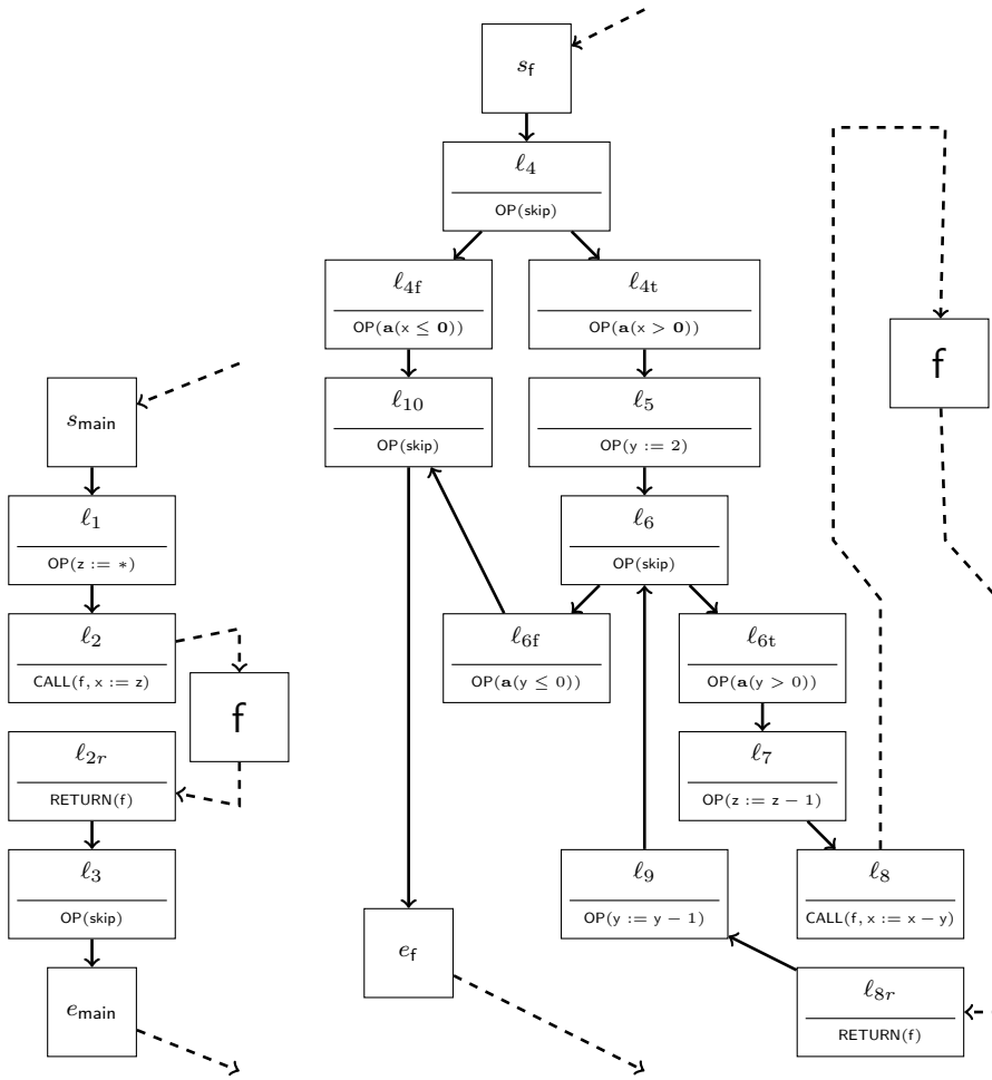
Fig. 2 Control-flow graphs for procedures main and f from Example 1. The notation \mathbf{a}(e) is shorthand for \mathbf{assume}(e) .
