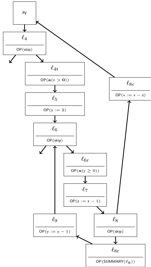
Fig. 7 Control-flow graph fragment from code of Example 5, after application of TOTALCFL.
