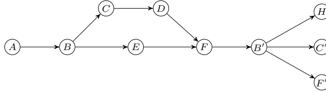
Fig. 1: DAG representation of AB[CD|E]FB'[H|C'|F']
